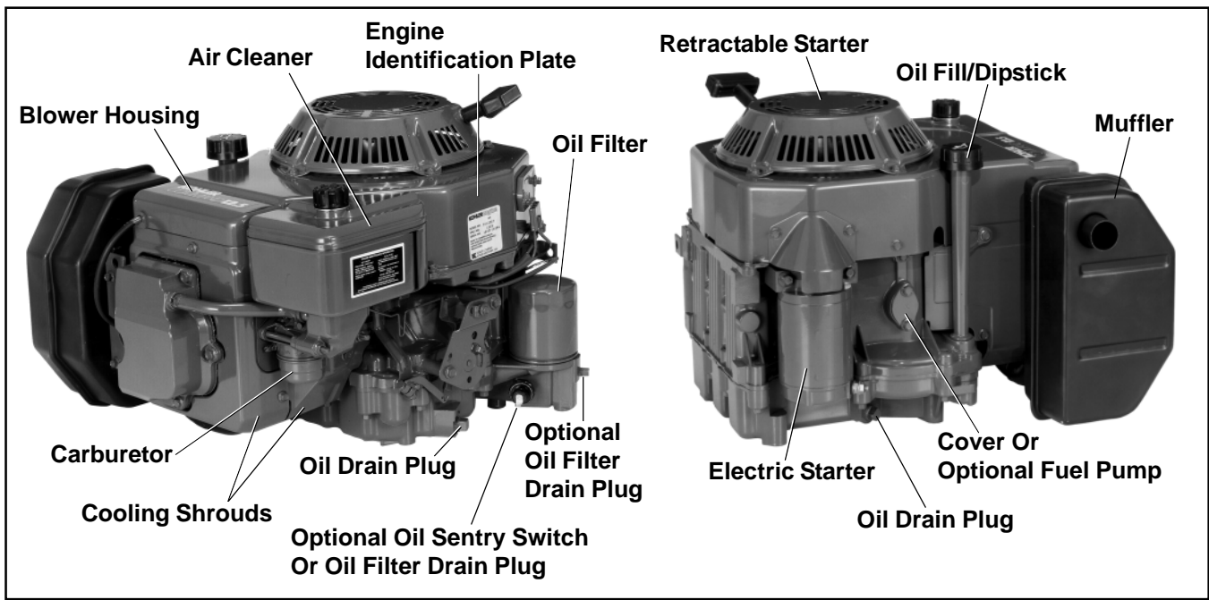
Figure 1. Typical Command Vertical Shaft Engine.
